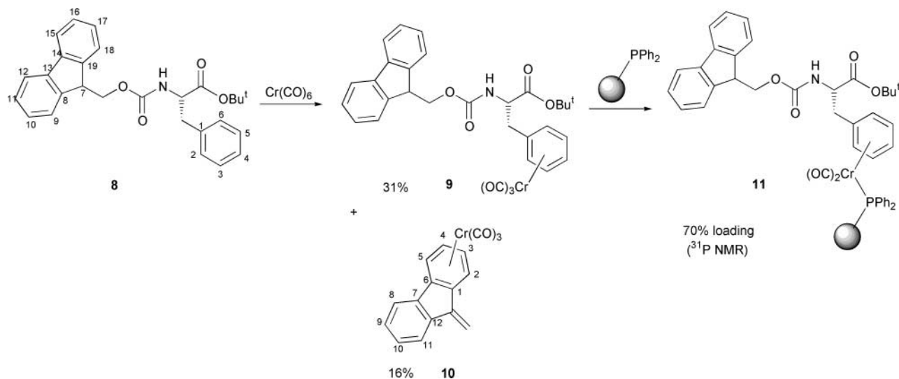
Scheme 3
